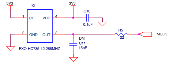
MCLK Oscillator
